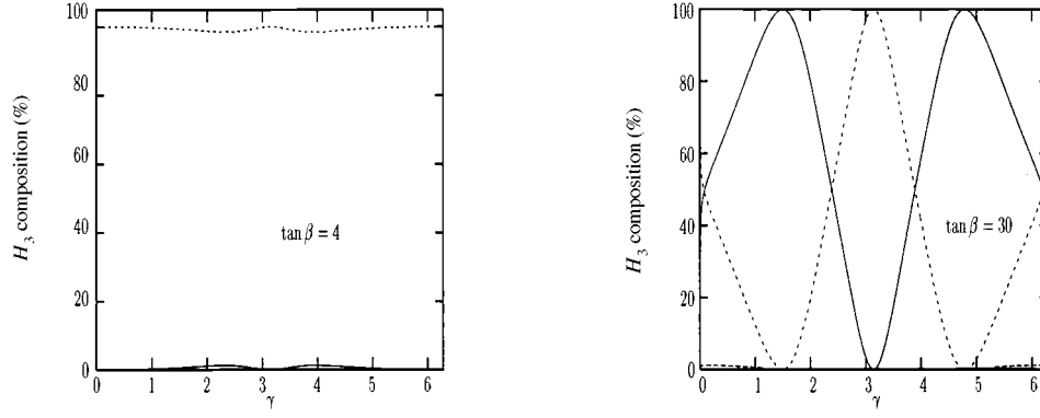
FIG. 4. Percentage composition of H_3 as a function of \gamma for \tan \beta = 4 (left panel) and \tan \beta = 30 (right panel). Here \phi_1 , \phi_2 , and \sin \beta \phi_1 + \cos \beta \phi_2 contributions are |\mathcal{R}_{31}|^2 (solid curve), |\mathcal{R}_{32}|^2 (dashed curve), and |\mathcal{R}_{33}|^2 (short-dashed curve), in percents.
