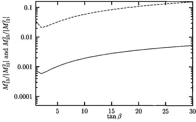
FIG. 1. Variation of M_{13}^2/M_{12}^2 (solid curve) and M_{23}^2/M_{12}^2 (dashed curve) with \tan\beta for M_{\tilde{L}}=M_{\tilde{R}}=|A_t|=10M_Z , |\mu|=2.5M_Z , and \tilde{M}_A=2M_Z with \gamma=\pi/4 . The CP -violating mixings become important for large \tan\beta .
