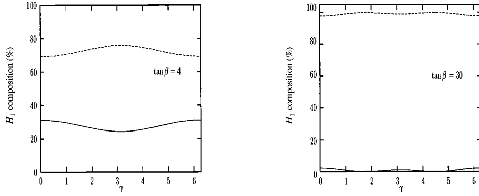
FIG. 2. Percentage composition of H_1 as a function of \gamma for \tan\beta=4 (left panel) and \tan\beta=30 (right panel). Here \phi_1 , \phi_2 , and \sin\beta\phi_1+\cos\beta\phi_2 contributions are |\mathcal{R}_{11}|^2 (solid curve), |\mathcal{R}_{12}|^2 (dashed curve), and |\mathcal{R}_{13}|^2 (short-dashed curve), in percents. Values of the parameters are given in Eqs. (29).
