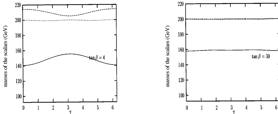
FIG. 5. Masses of the scalars H_i as a function of \gamma for \tan \beta = 4 (left panel) and \tan \beta = 30 (right panel). Here M_{H_1} , M_{H_2} , and M_{H_3} are shown by solid, dashed, and short-dashed curves, respectively. In both panels H_1 is the lightest scalar whose composition is shown in Fig. 2.
